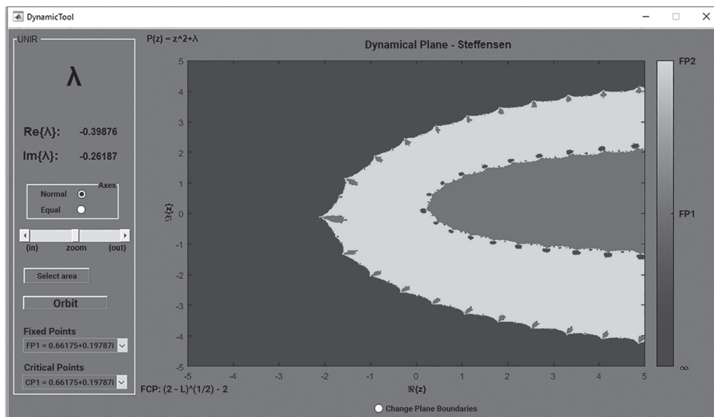
GRAPH 5. “DynamicTool” GUI in action.
