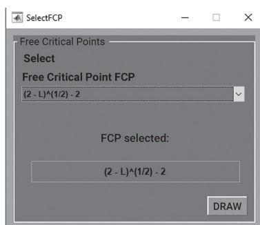
GRAPH 6. “SelectFCP” GUI.
